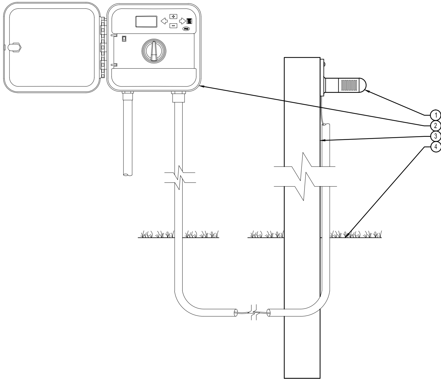
XX FREEZE-CLIK WITH GENERIC WALL MOUNT CONTROLLER Monter S.FC.01
